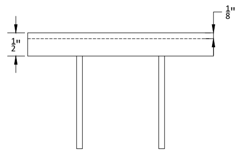
2 MEDALLION SECTION NTS
