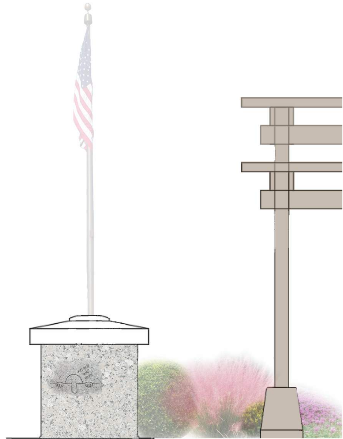
SIDE OF US FLAG PEDESTAL + RELATION TO PERGOLA
